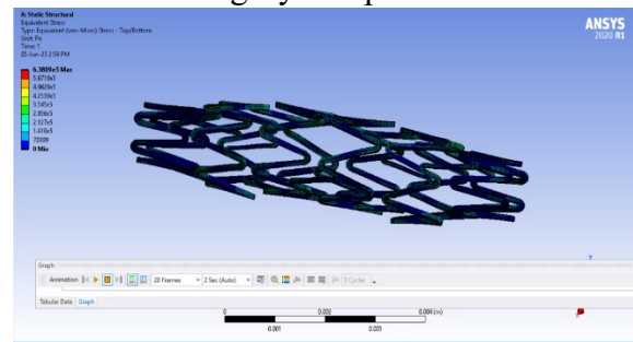
Figure 4 Equivalent von mises stress of stent design 2
