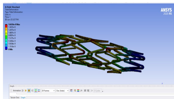
Figure 8 Total deformation of stent design 2
