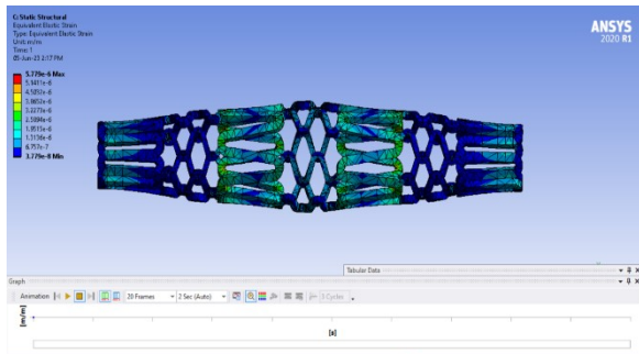
Figure 5 Equivalent von mises strain of stent design 1
