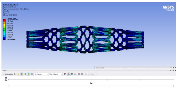
Figure 3 Equivalent von mises stress of stent design 1
