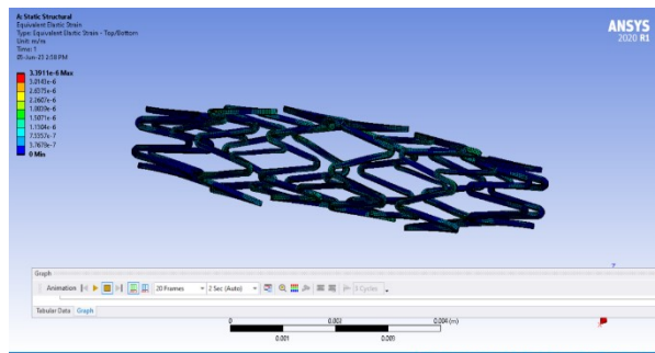
Figure 6 Equivalent von mises strain of stent design 2
